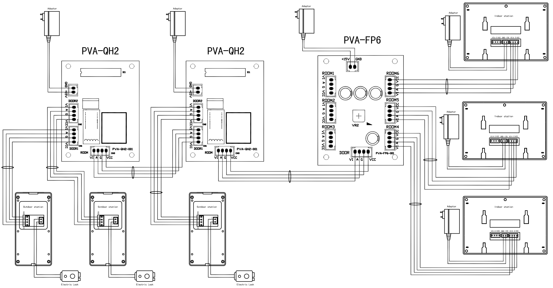
Three to Three Video Door Phone Wiring Diagram
